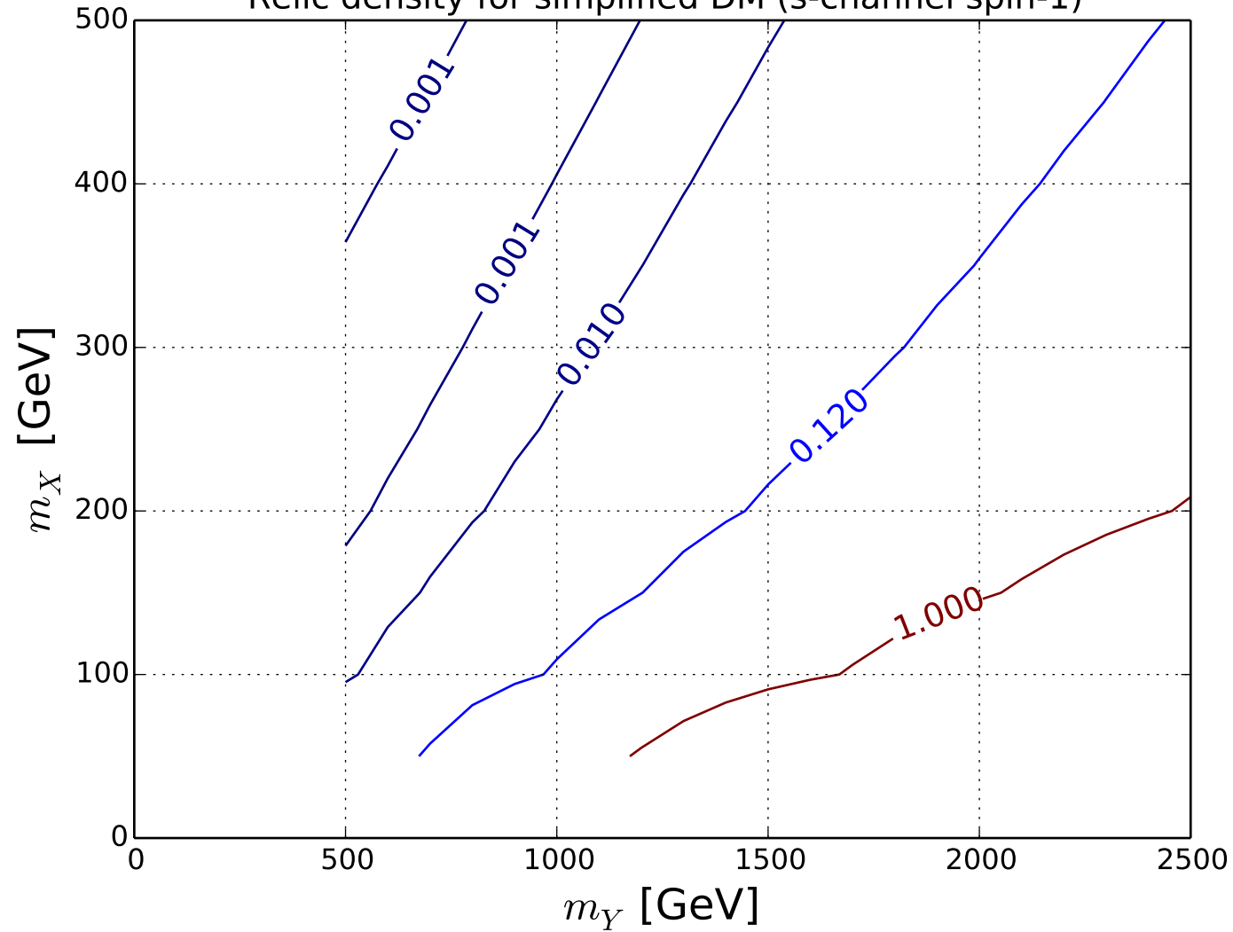
Relic density for simplified DM (s-channel spin-1)
